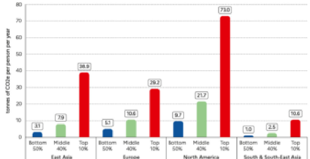
Figure 15 Per capita emissions across the world, 2019
